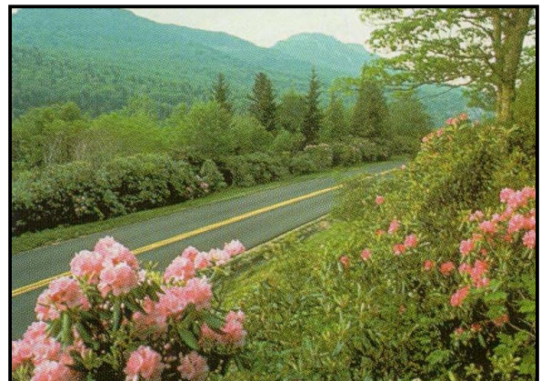
Rank - #3 Score - 8.41
